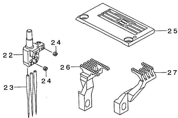
MF-7723-U10-B56
